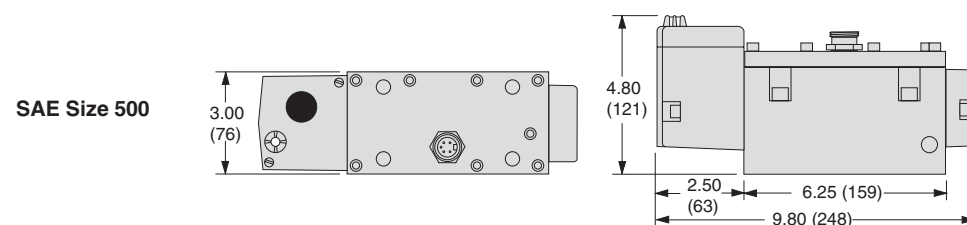
Ford Wired 5-pin mini-connector (all voltages)
